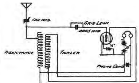
Fig. 4. Circuit Used.
