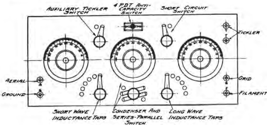
Fig. 2. Completed Panel.
