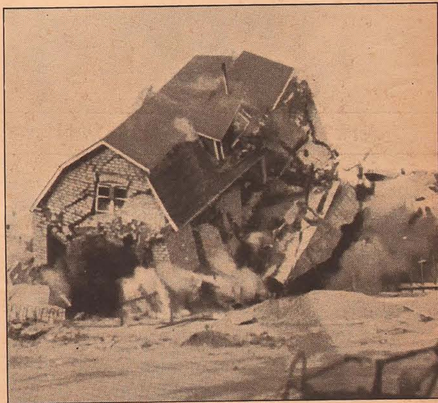
Extensive use is made of dynamite in tearing down old buildings to be replaced by new ones. In blasting the old lifeguard quarters (above) at Orchard Beach, Pelham Bay Park, New York, 60 pounds of dynamite was used
