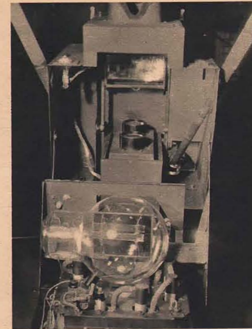
29 Inside the camera, center, is the iconoscope, or "television eye." The plate inside tube changes light to electrical waves
