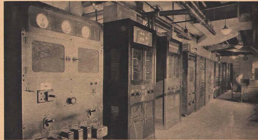
25 Half the units shown above are audio (sound) transmitters, half video (pictures). In the pipes, audio and video signals are combined in an antenna filter. Thus simultaneous sound and picture transmission is possible. Program is piped to antenna—then into air
