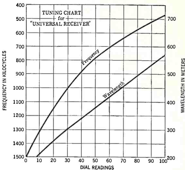
A TUNING CHART FOR THE "UNIVERSAL"
