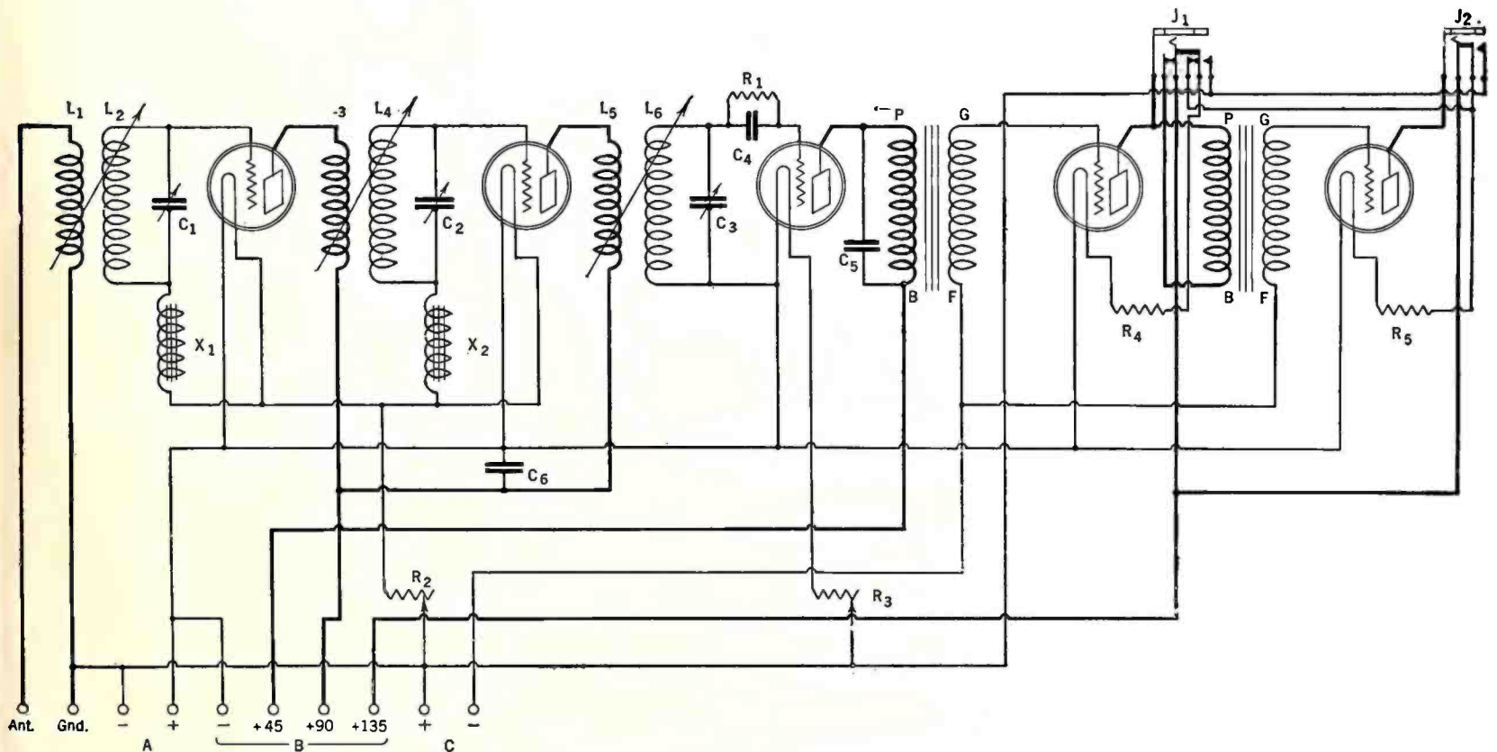
A FIVE-TUBE CIRCUIT
