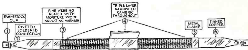
"THE SIX-POINT LEAD-IN"
