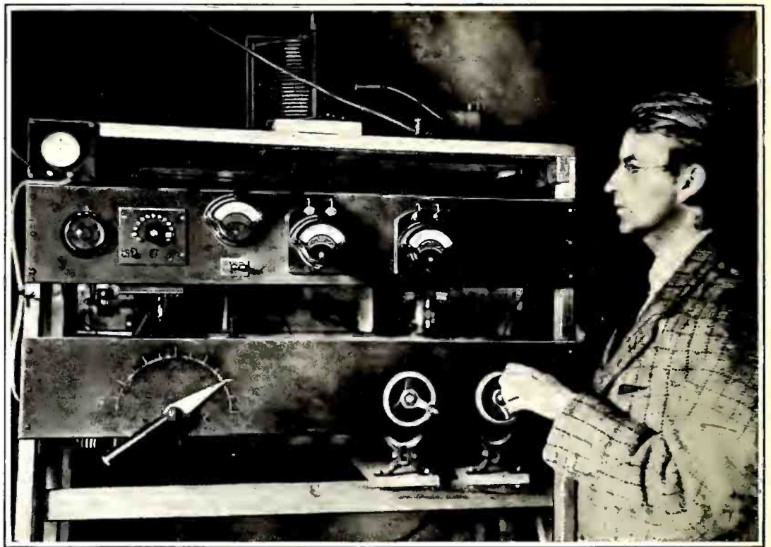
THE TRANSMITTING APPARATUS
