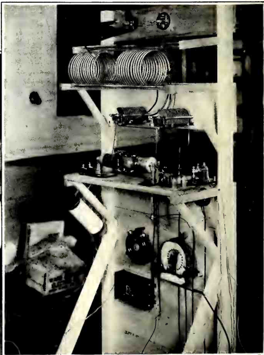
—Port Arthur, Ontario. This 250-watt station (C-9AQ) works with the base station, 600 miles away at Toronto (C-9A1). In daytime a frequency of 10,000 kc. (29.94 meters) is used and at night 5906 kc. (50 meters). The Cameron Falls power station supplies the twin cities of Fort William and Port Arthur with electric power
