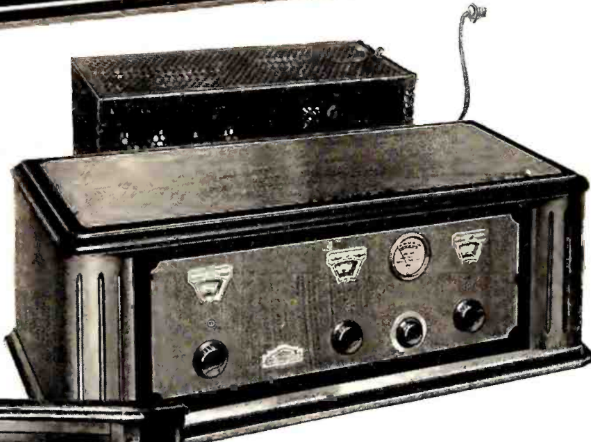
5-Tube Lamp Socket Model AC-5
