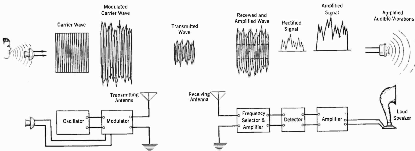
HOW SOUND WAVES ARE BROADCAST AND RECEIVED
