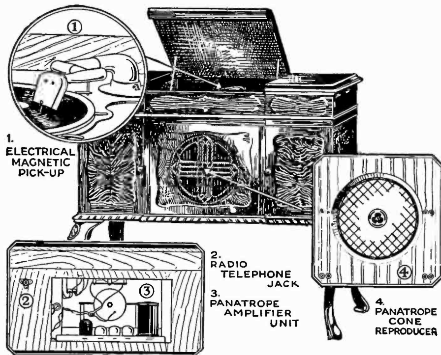
THE PANATROPE
