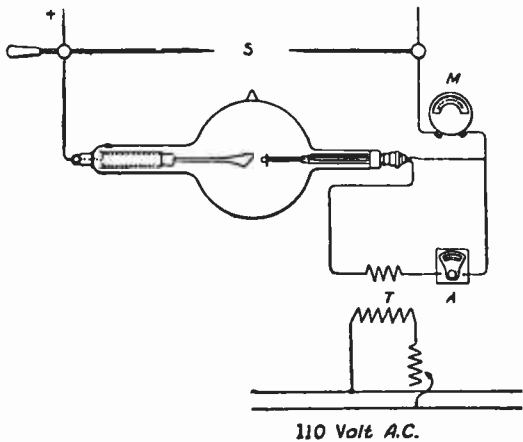
COOLIDGE X-RAY TUBE WIRING
