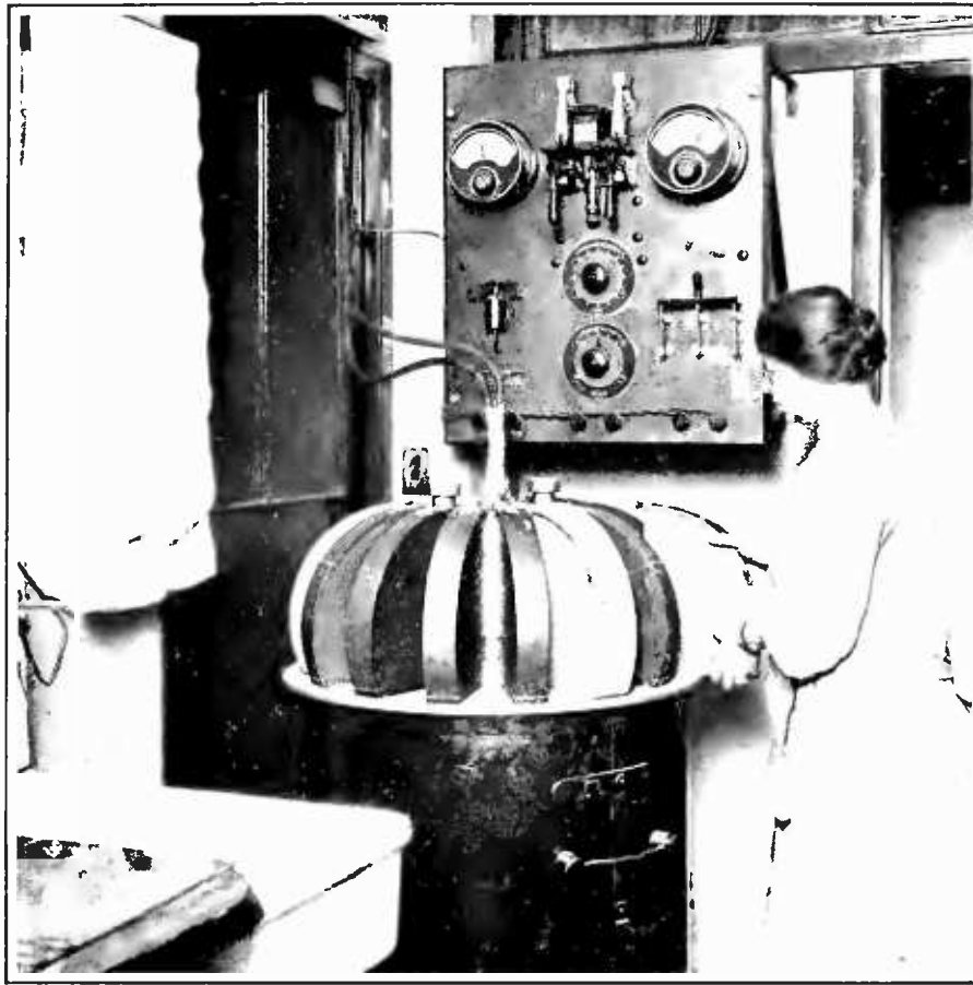
X-RAY DIFFRACTION APPARATUS
