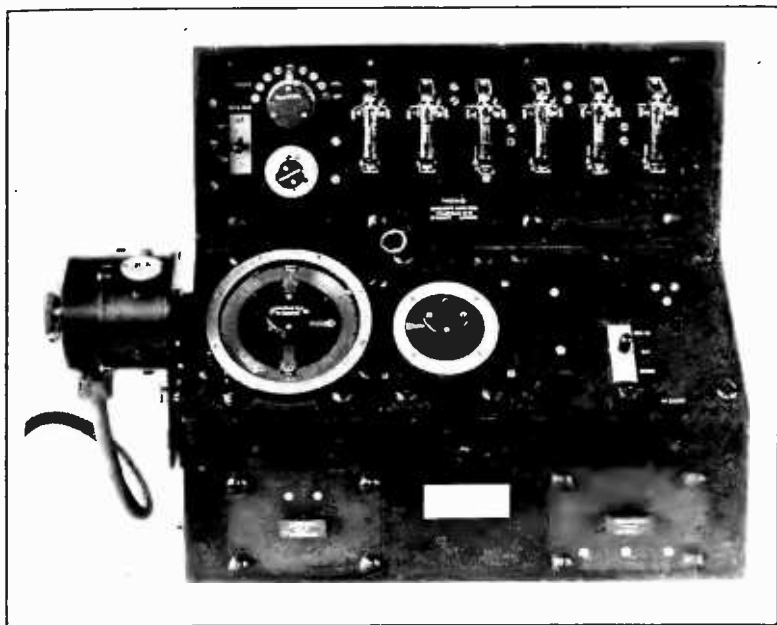
ENGLISH DIRECTION-FINDING EQUIPMENT
