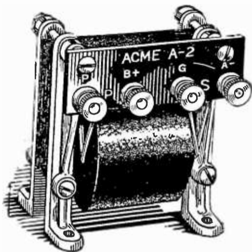
Acme A-2 Audio Frequency Amplifying Transformer
