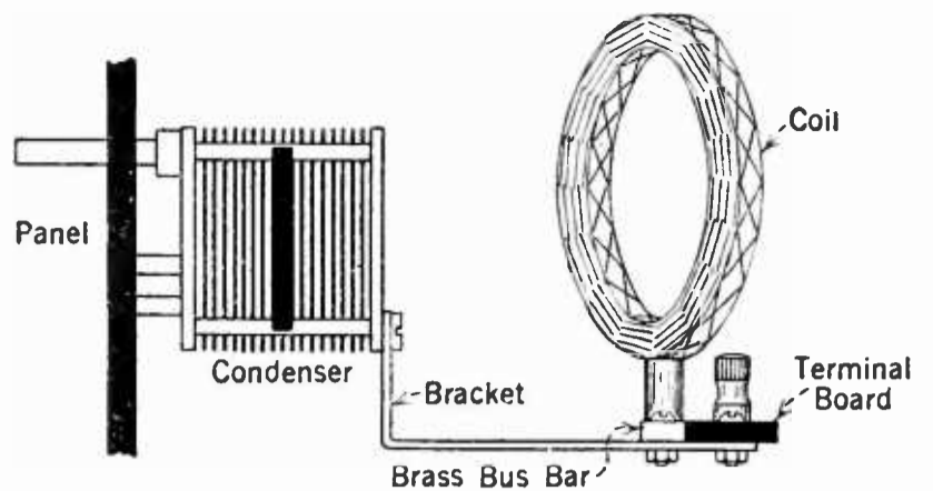
METHOD OF ASSEMBLY OF CONDENSER, ANGLE BRACKET, COIL AND TERMINAL BOARD
