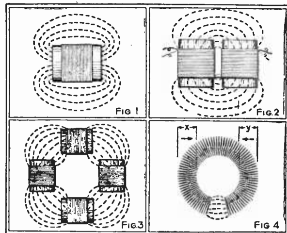
General Theory of the Toro-Tran
