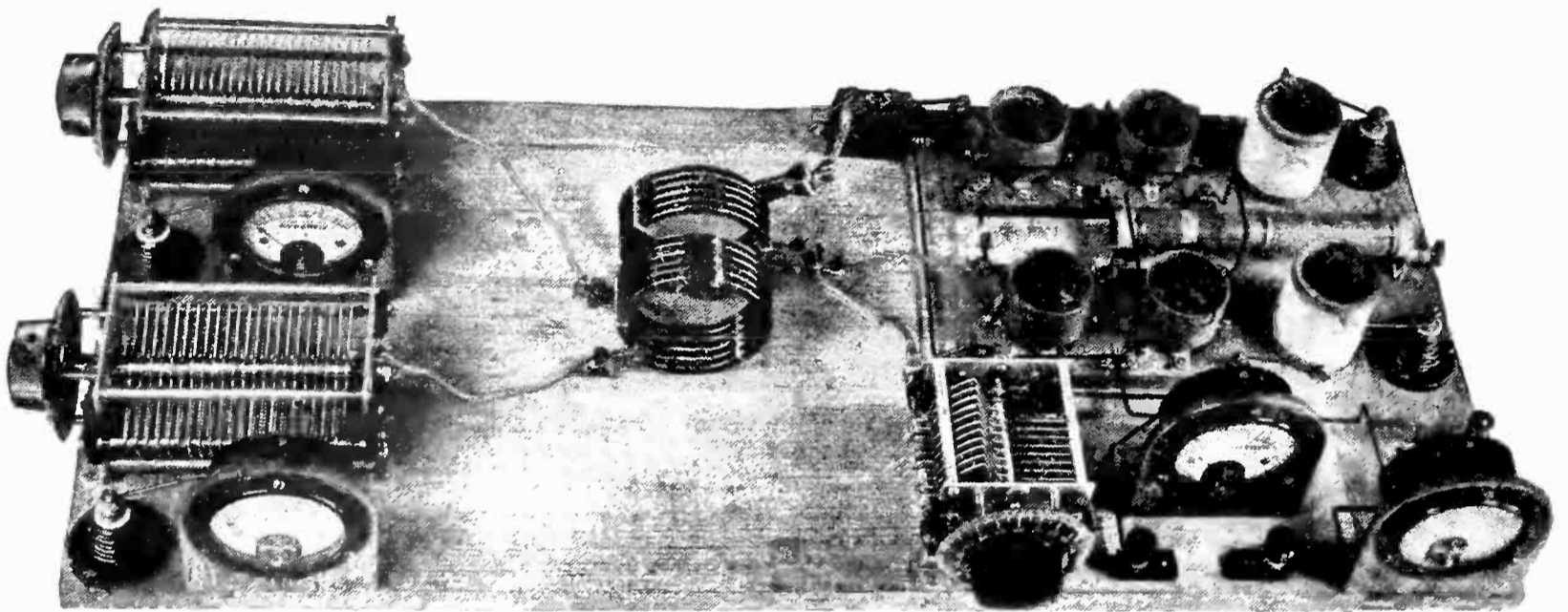
LIEUT. SCHNELL'S TRANSMITTER USING THREE NATIONAL CONDENSERS
