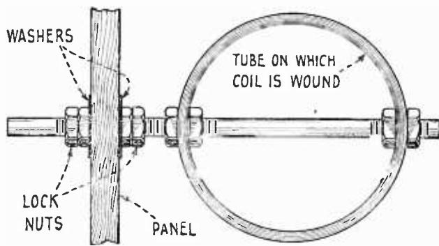
FIG. 2 Showing bearing for movable coils
