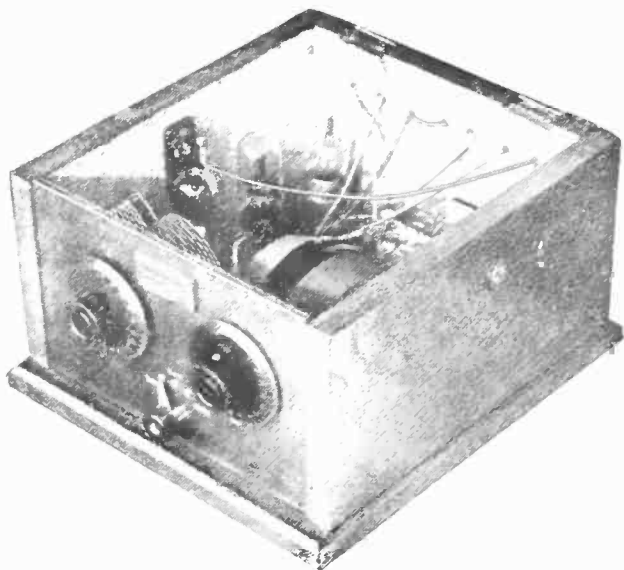
A 3-TUBE SET IN A SMALL SPACE
