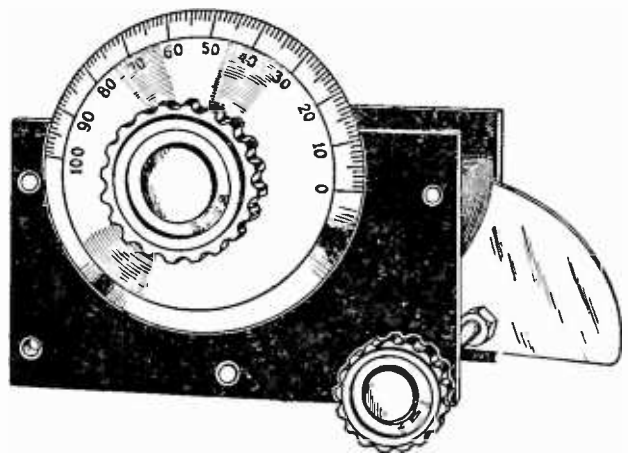
PLATE VERNIER
