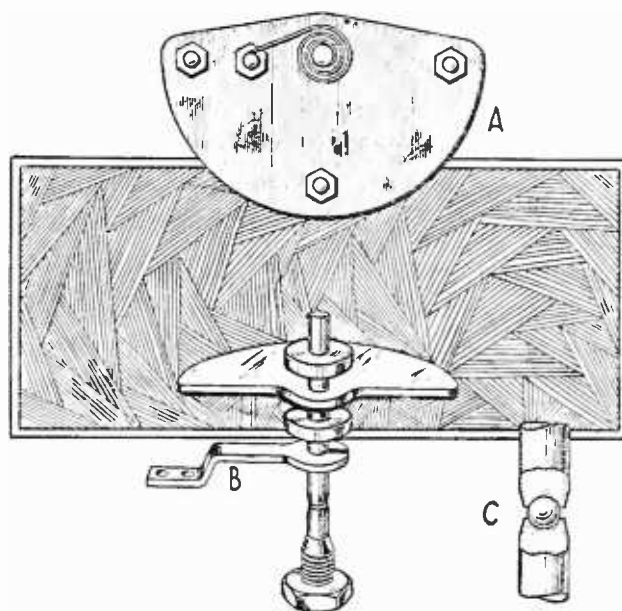
THREE TYPES OF ROTOR CONNECTIONS
