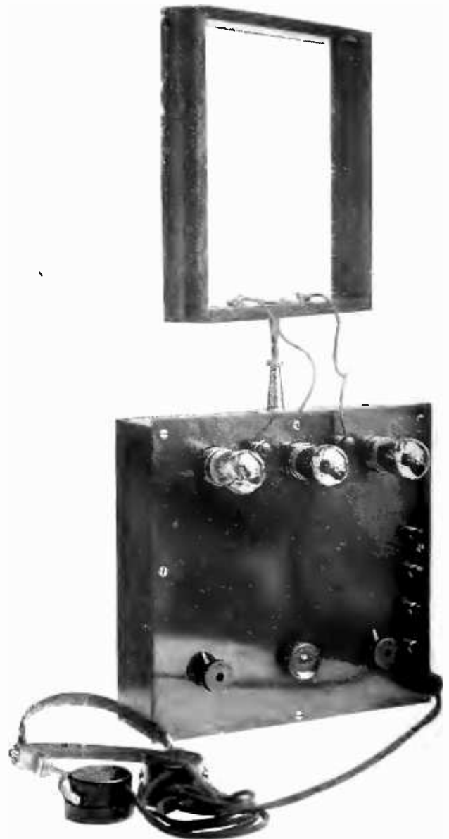
THE COMPLETE "INVERSE DUPLEX" RECEIVER One of these sets has been tried out by the Editor of RADIO BROADCAST. The first night, he heard, from his home on Long Island, PWX (Havana, 1300 miles) and WDAF (Kansas City, 1080 miles)
