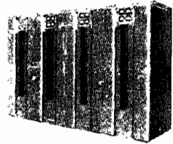
A four-kilowatt Farnsworth television picture transmitter.
