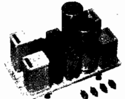
The 111-A Amplifier consists of two individual pre-amplifiers on a single chassis for use in high quality speech input equipment. Its compact unitized construction saves rack space. Input impedances of 30, 250 and 600 ohms; output impedance 600 ohms. It is quiet and has excellent frequency characteristics and ample power output with low distortion products.
