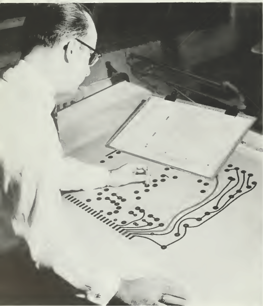
1. Process begins with preparation of a large production photo-master of the original circuit drawing. Here photo-master is copied from small drawing at top.
