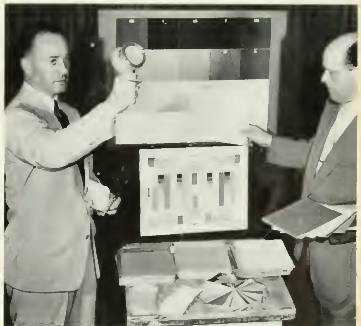
The author (left) measures the temperature of the studio illumination as Cliff Stiegelbauer holds a red-orange card against a gray scale. The comparison shows that this particular hue will be reproduced on TV screens as Munsell \approx 7 gray.
