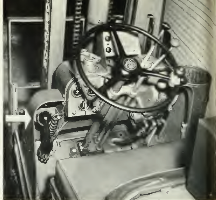
Headsets for the fork lifts are placed at the left of the operator with the transmitter-receiver installed behind the seat (extreme right).
