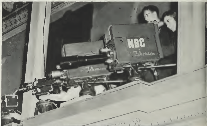
RCA IMAGE ORTHICON CAMERAS INSTALLED IN GALLERY OF THE HOUSE OF REPRESENTATIVES ARE TRAINED ON THE SPEAKER'S STAND.
