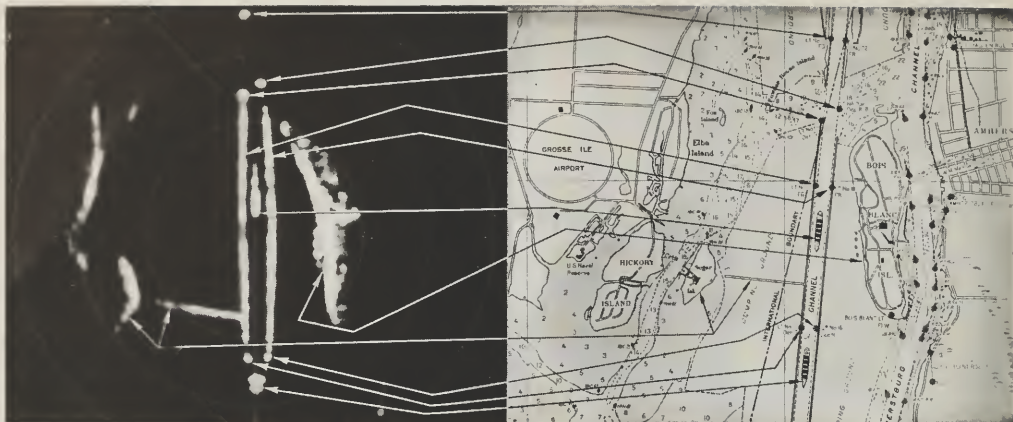
Radiomarine's Radar Scope Picture (approximately \frac{1}{4} actual size). 1\frac{1}{2} -mile range.
