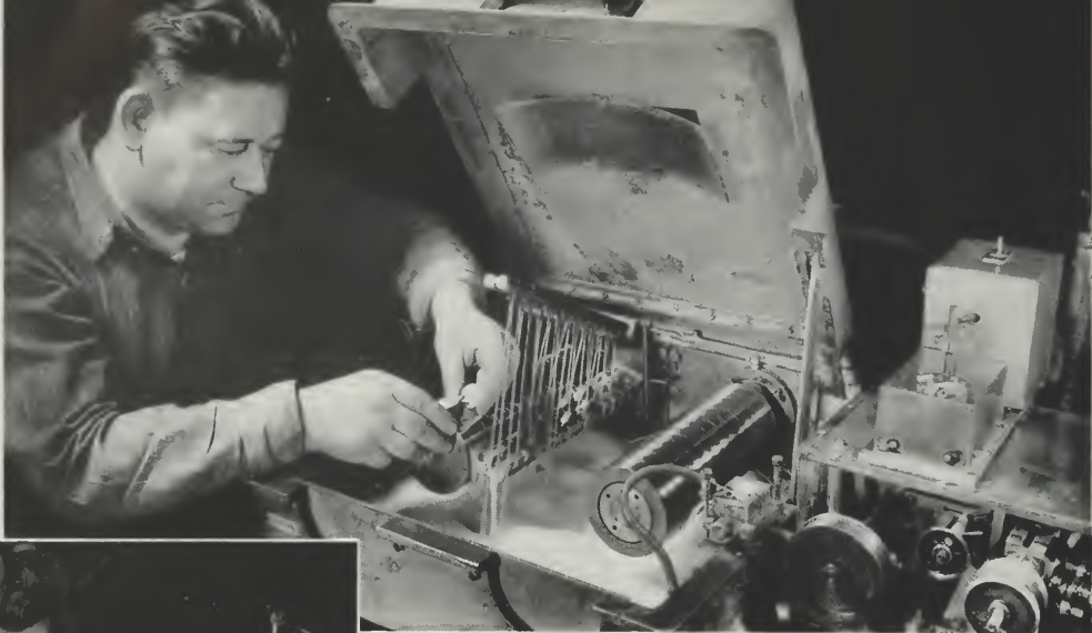
FILAMENTS FOR MINIATURE TUBES ARE MADE BY RUNNING WIRE AS FINE AS SILK THROUGH THE DIAMOND DIES OF THIS MACHINE WHICH REDUCES THE WIRE DIAMETER TO ONE THIRD THE THICKNESS OF HUMAN HAIR.
