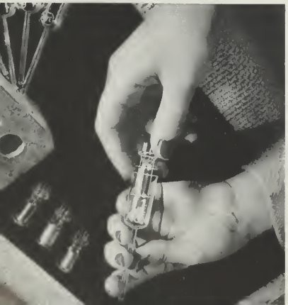
SLIDING A GLASS ENVELOPE WITH EXHAUST TUBE ATTACHED OVER THE ELEMENTS OF A MINIATURE TUBE.
