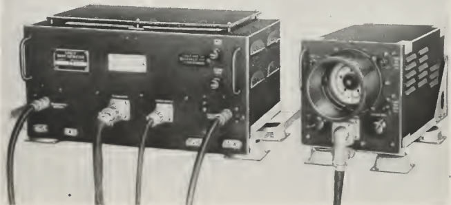
COMPLETE ALTIMETER INSTALLATION DESIGNED BY RCA TO COVER ANY ALTITUDE NORMALLY REACHED BY AIRPLANES.
