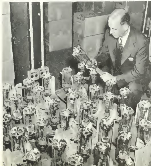
BOTTOM — THE JOB OF REBUILDING THEM COMPLETED, A GROUP OF TUBES ARE MADE READY FOR PACKING AND SHIPPING TO BROADCASTING STATIONS.
