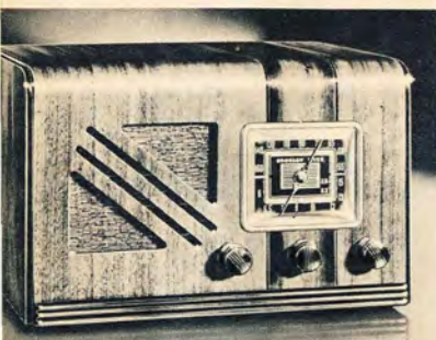
CROSLLEY FIVER—20AP. Five tubes, six-inch dynamic speaker, loop antenna, large "Gold Glow" dial, automatic volume control. Hand-rubbed walnut cabinet, protected by the Crosley Jewel Case Protector. $19.99
